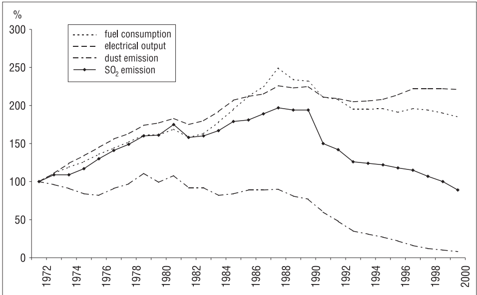
Fig. 1. Pollutant Emissions in Public Power Utilities vs. Fuel Consumption and Electricity Generation (1971=100)
