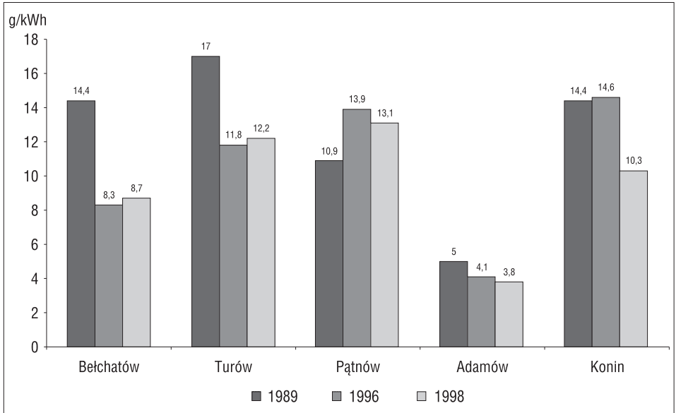
Fig. 4 Unit SO 2 Emissions in Brown-Coal Fired Plants in 1989, 1996 and 1998.
