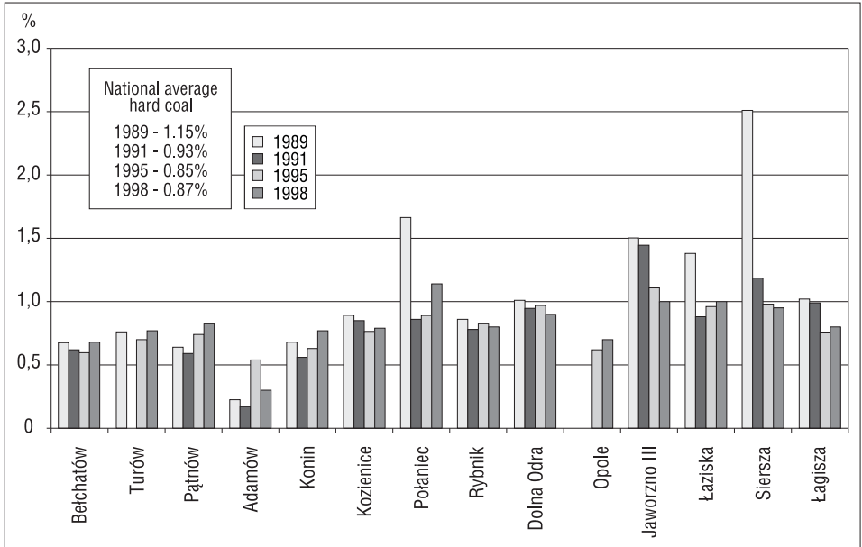
Fig. 5. Sulphur Content in Hard Coal Used by Power and Combined Heat and Power Plants Larger Than 700 MW
